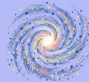
6. Galaxy
